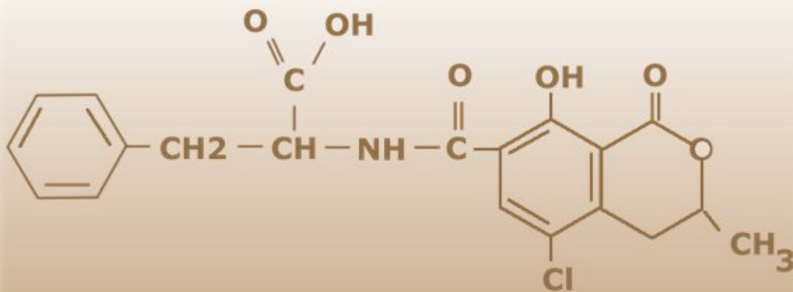
Ochratoxin A
