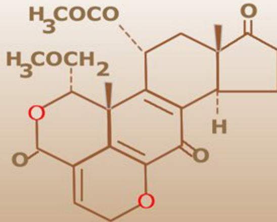
Chemical structure of Wortmannin
